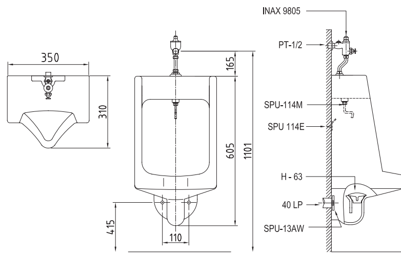
U-114N urinal
