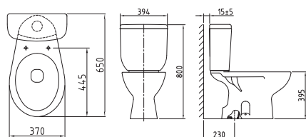
C-65 / T-950N wash down system
