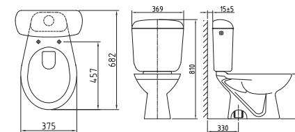
C-19 / T-108 wash down system
