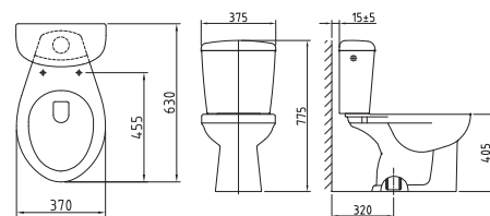
C-30 / T-30 wash down system
