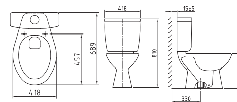
C-21 / T-21 wash down system
