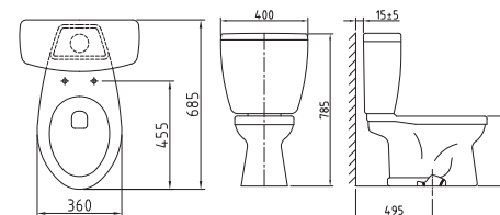
C-20 / T-20 wash down system
