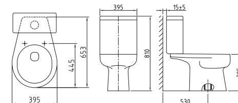
C-68 / T-68 wash down system
