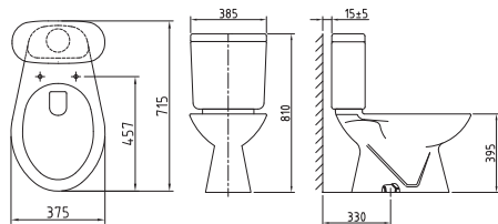
C-22 / T-22 wash down system
